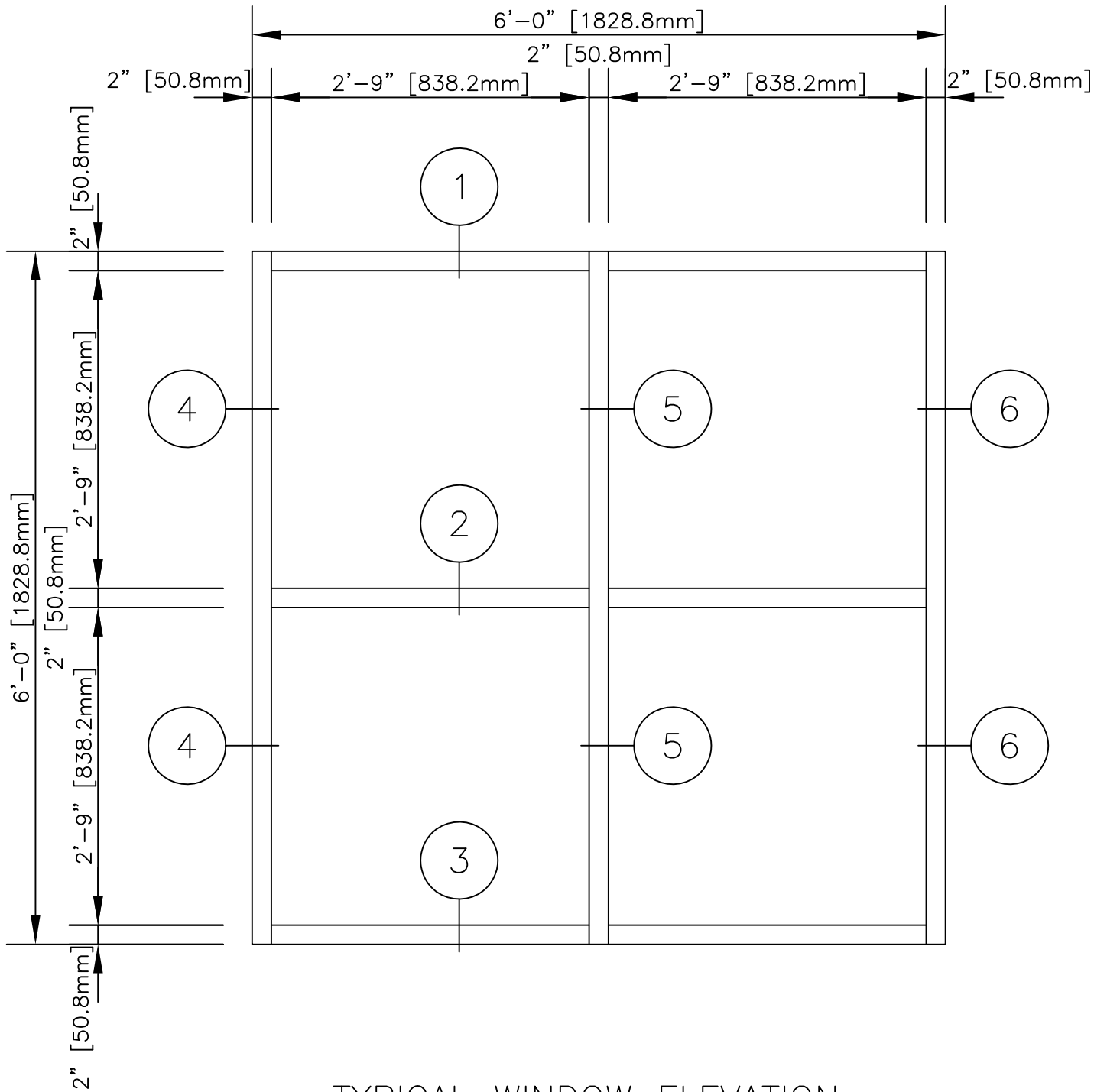
TYPICAL WINDOW ELEVATION
